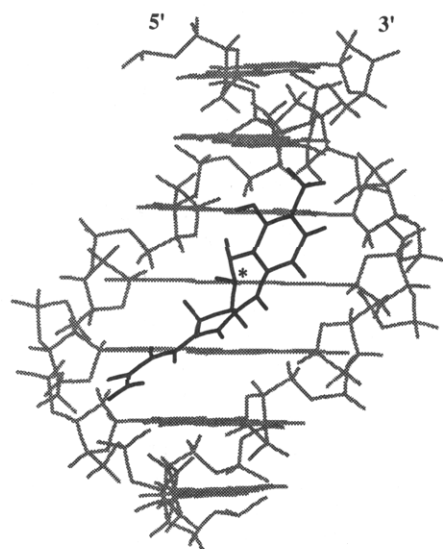
Figure 2. Model of anthramycin covalently linked [through a C11( S ) bond] to the N 2 of a guanine residue (marked with *) within the minor groove of B-form DNA (A ring oriented toward the 3'-end of the covalently-modified strand; model is not energy minimized).
